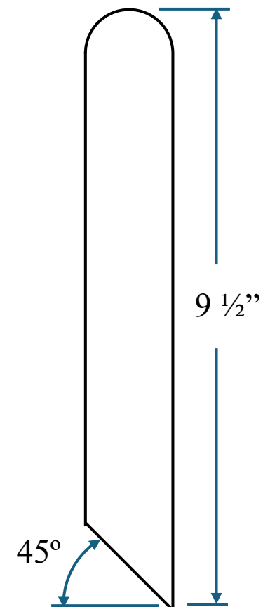
Piece 6 Angled Support Board 4 required
