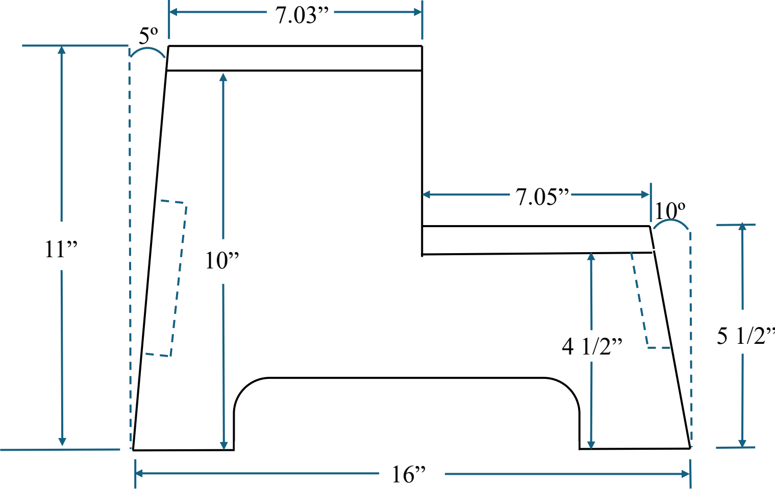
Side View
