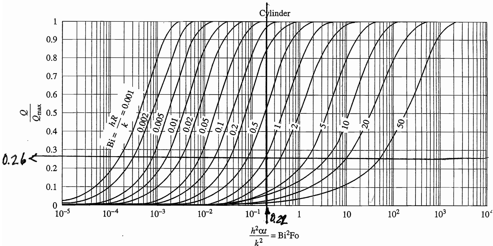
Figure 5-11 Total heat transfer between an infinite cylinder and the surrounding fluid. (Drawn from [4] with permission.)
