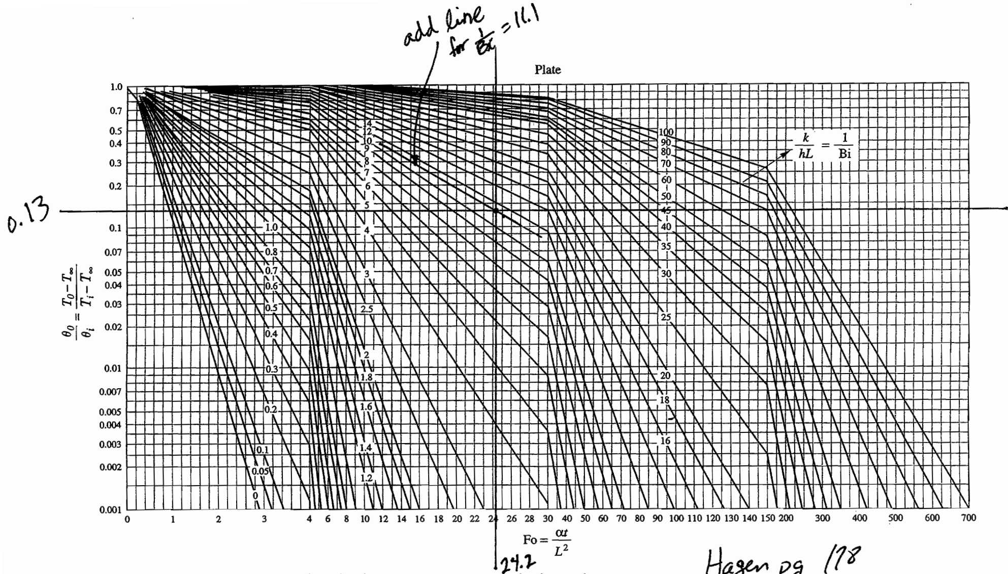
Figure 5-6(a) Temperature response chart for the center temperature of infinite plates. (Drawn from [2] with permission.)
