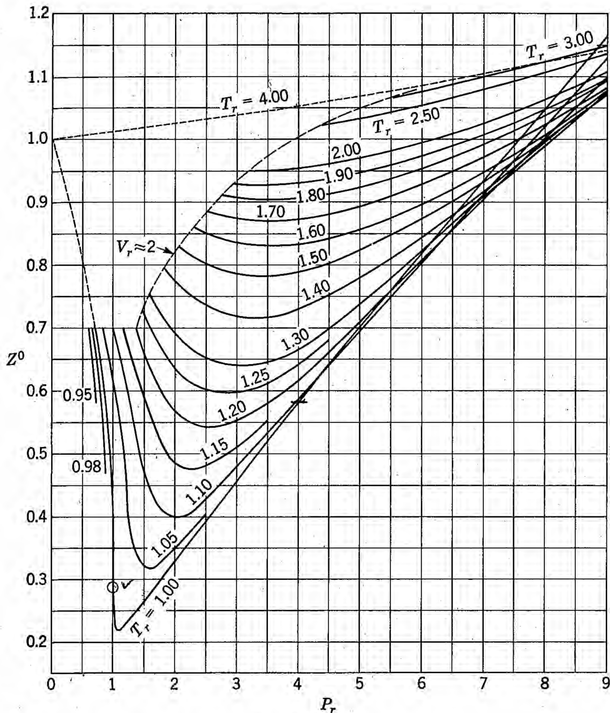
Fig. 3-12 Generalized correlation for Z^0 . Based on data for argon, krypton, and xenon from Pitzer's correlation.
