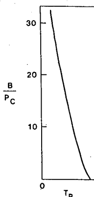
Figure 1. COSTALD B/P_c ; \omega_{SRK} = 0.1584 .
